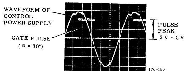
Fig. 26 Gate Pulse Waveforms
