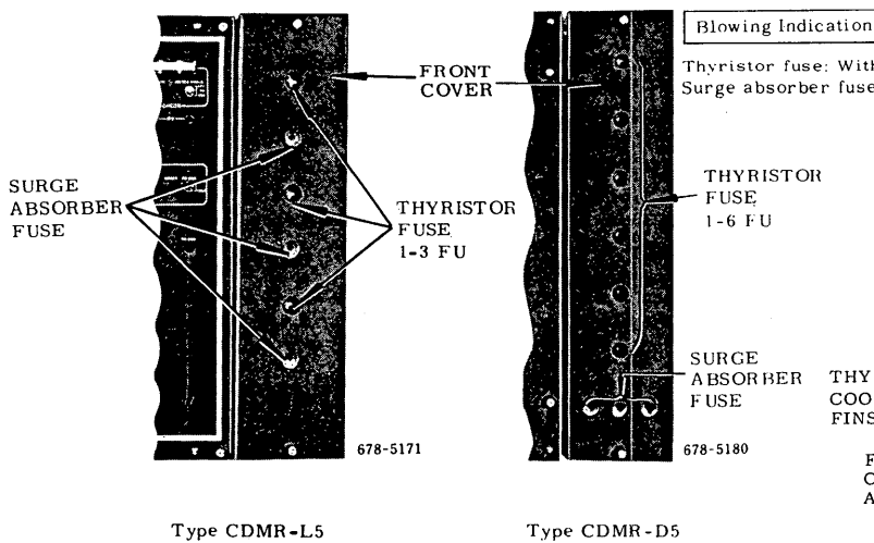
Fig. 15 Fuse Locations
