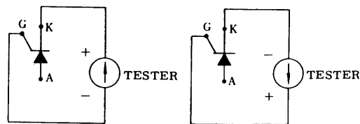
Fig. 28 Testing Module by Connecting Tester across A and K
