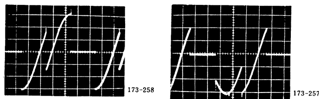
Fig. 27 Thyristor Voltage Waveforms across Terminals A-K
