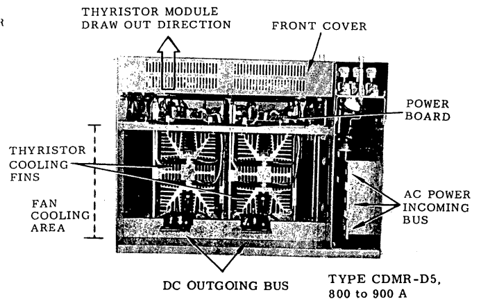
Fig. 16 Ventilating System Viewed from Bottom of the Unit
