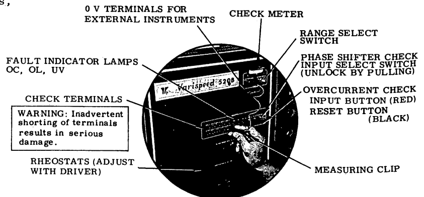
Fig. 8 Front Panel Arrangement
