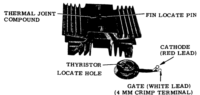
Fig. 21 View After the Removal of Thyristor
