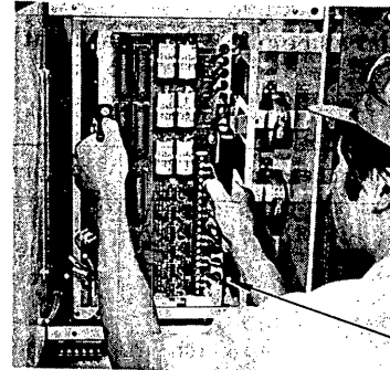
Fig. 19 Dismounting Thyristor Modules
