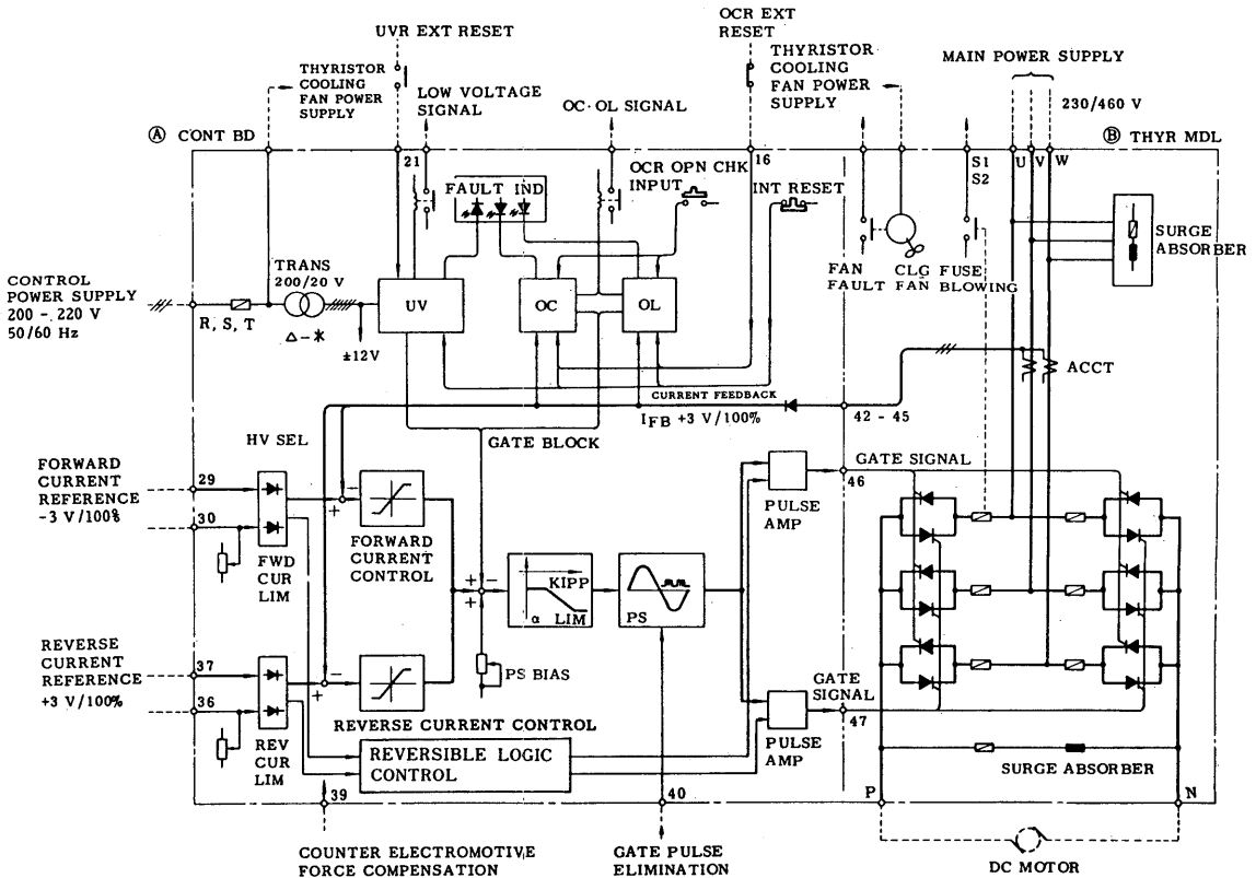
Fig. 1 Type CDMR-L5 Single Converter
