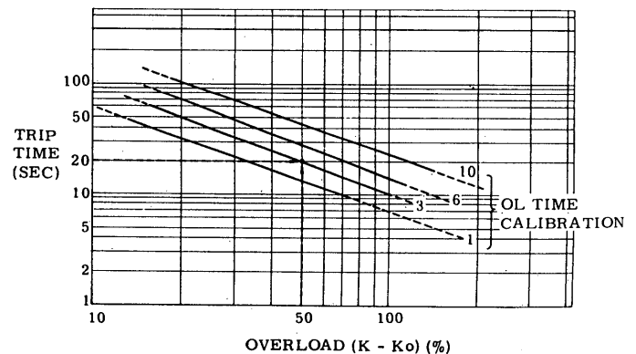
Fig. 13 Overload-trip Time Characteristics
