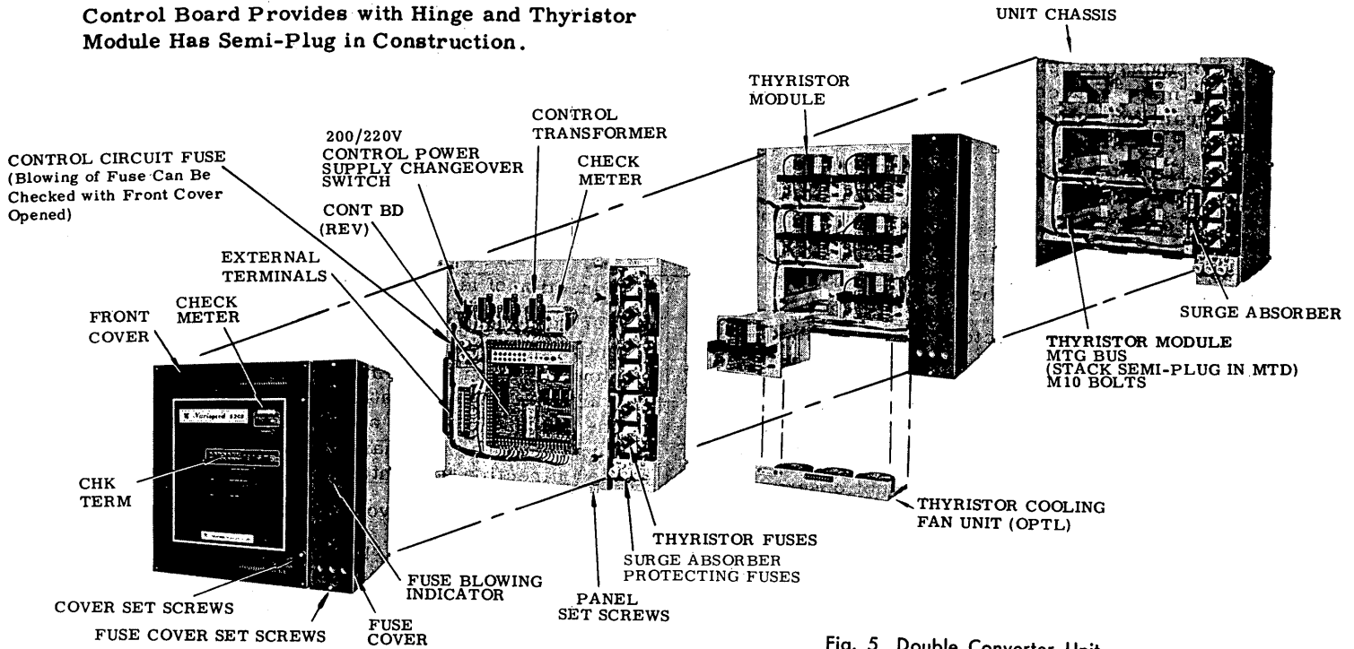
Fig. 5 Double Converter Unit
