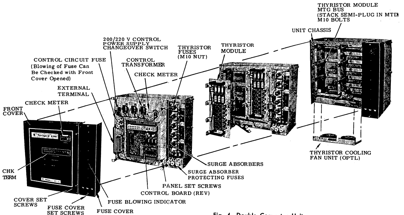
Fig. 4 Double Converter Unit
